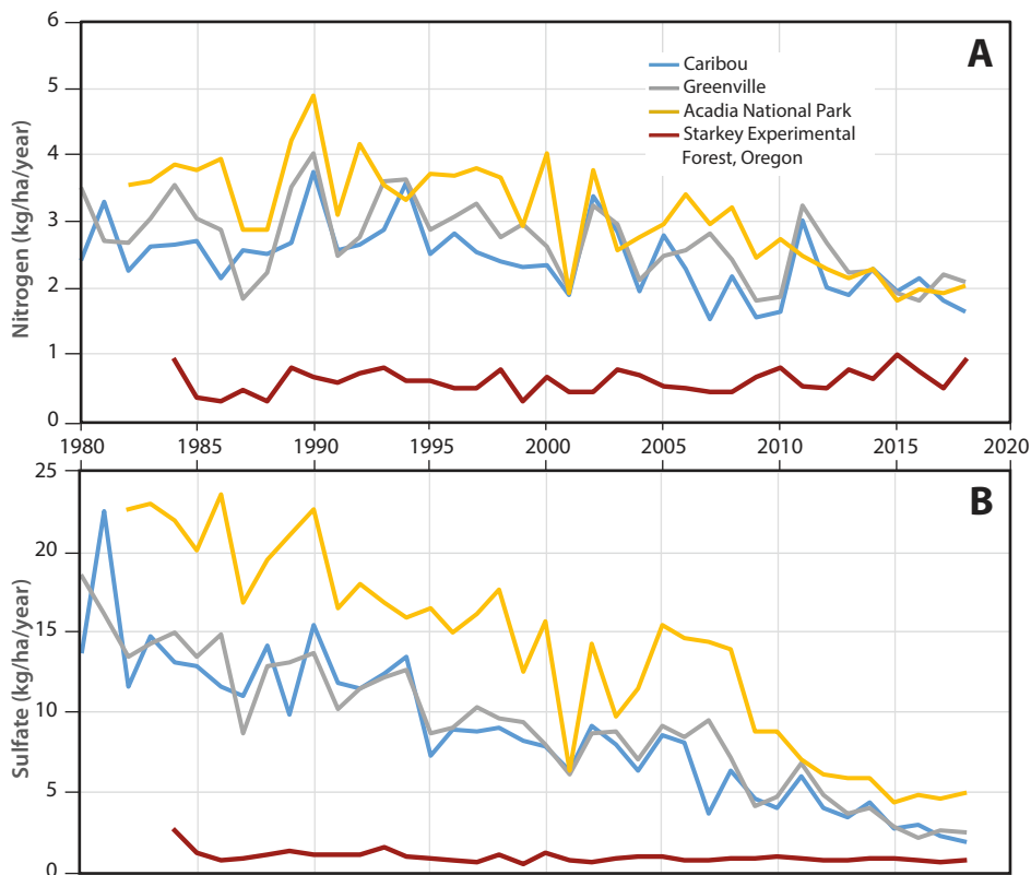
Total annual wet-only inorganic nitrogen (A) and sulfate (B) deposition, from three Maine monitoring stations in the National Atmospheric Deposition Program (NADP). Data from an Oregon monitoring station (without upwind pollution sources) shown for contrast.
