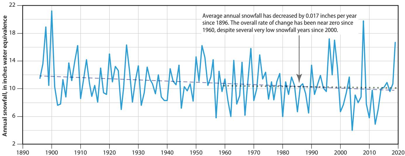
Maine Annual Snowfall, 1896–2019
